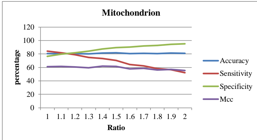
Supplementary figure 6 Negative and positive ratio test in Mitochondrion by SVMs
