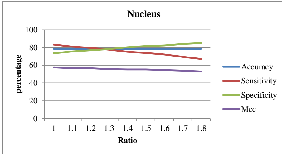
Supplementary figure 7 Negative and positive ratio test in Nucleus by SVMs
