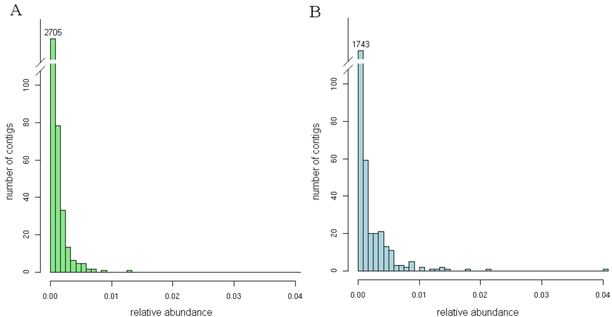
Supplementary Figure 3S. Distribution of clustered sequences from sporulation (A) and germination (B) stages of B. emersonii life cycle. The vertical axis of the normalized histogram shows the number of contigs. The horizontal axis shows the abundance ranges. Singlets were also considered for histogram construction. The number of contigs was normalized taking into account the total amount of accepted sequences in each developmental stage
