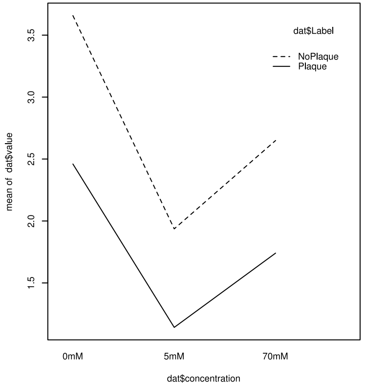
S6 Fig. Interaction analysis Labels (plaque/no plaque) and potassium concentration. A) Boxplots showing values based on label (plaque/no plaque) and potassium concentrations. B) Interaction plots displaying the levels of one factor on the x-axis and the mean response on the y-axis.
