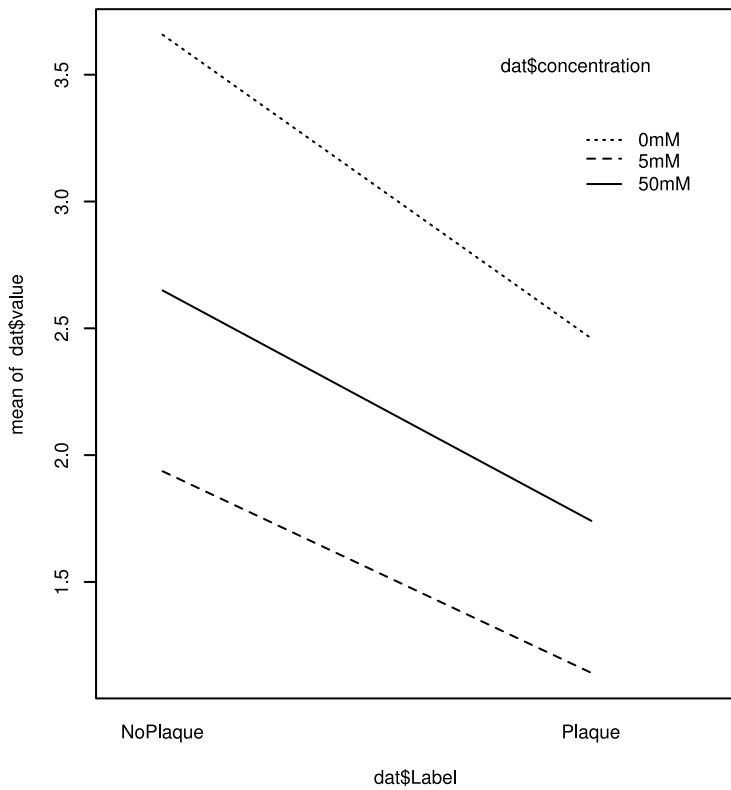
S6 Fig. Interaction analysis Labels (plaque/no plaque) and potassium concentration. A) Boxplots showing values based on label (plaque/no plaque) and potassium concentrations. B) Interaction plots displaying the levels of one factor on the x-axis and the mean response on the y-axis.
