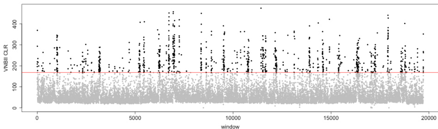
Supplemental Fig S6. Genome-wide signatures of selection across each of lineages VNI, VNBI, and VNBII. Values were computed using the composite likelihood ratio (CLR) test across windows of 50 segregating sites. Red lines indicate the top 5% of CLR values for each lineage; points above those lines are shown in black, while points below those lines are shown in grey.
