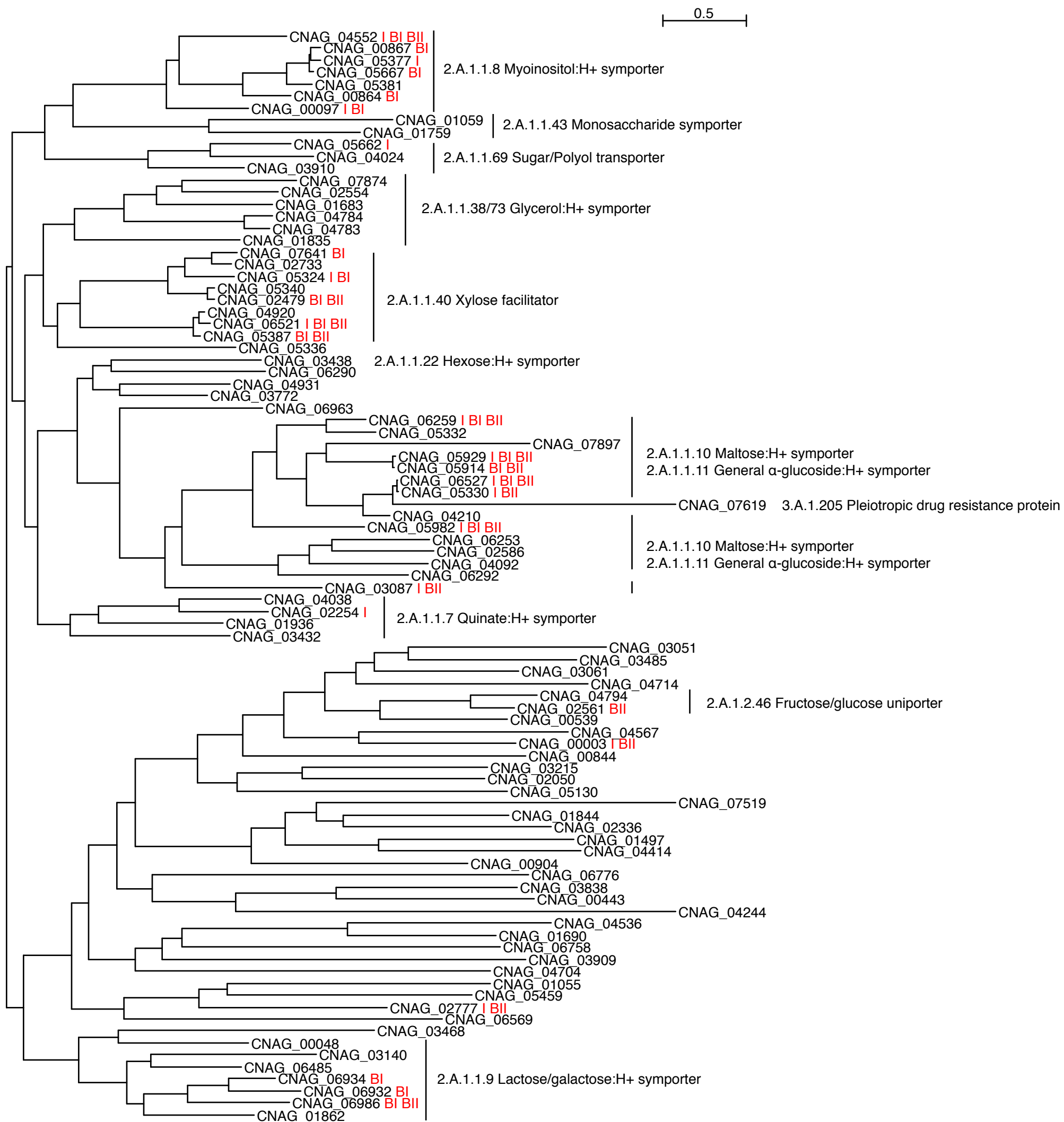
Supplemental Fig S7. Phylogenetic analysis of sugar transporters in the reference strain H99. Genes under selection in each lineage are labeled in red. Genes were annotated by best BLAST hits to the transporter classification database ( http://www.tcdb.org/ ).
