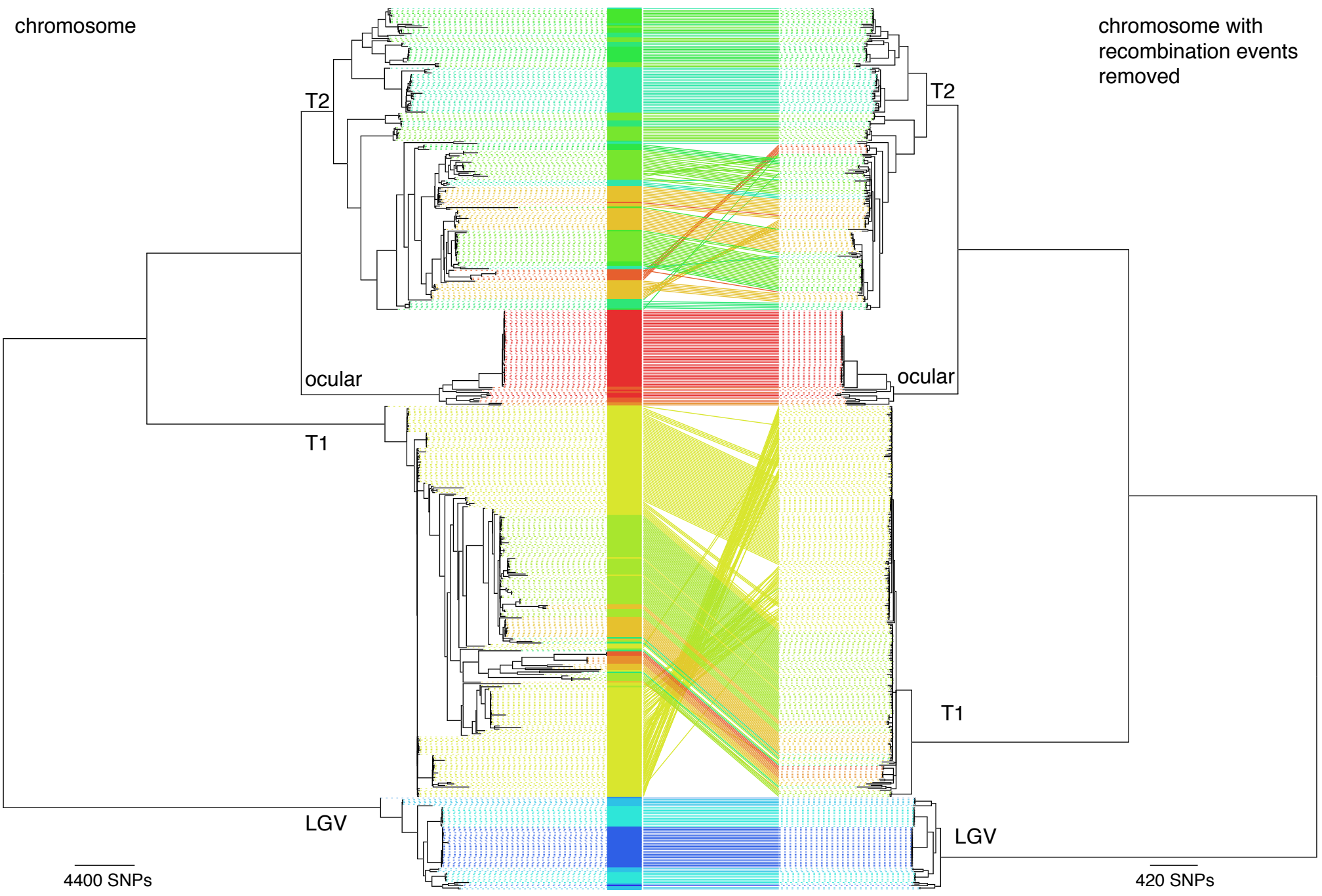
Supplemental Fig S4 Tanglegram of maximum-likelihood trees between chromosome (left) and chromosome with recombinations removed (right). Scale bars show single nucleotide polymorphism (SNP) differences and are specific to each tree.
