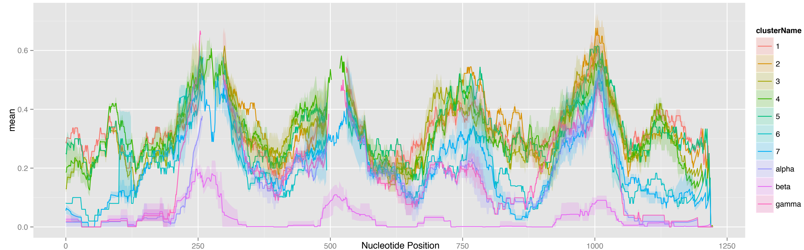
Supplemental Fig S6 Pairwise comparison of major outer membrane protein (MOMP) clades found in Figure 5C with L1_404 (the most ancestral Chlamydia trachomatis isolate obtained in 1967). Shading shows 10th and 90th percentile.
