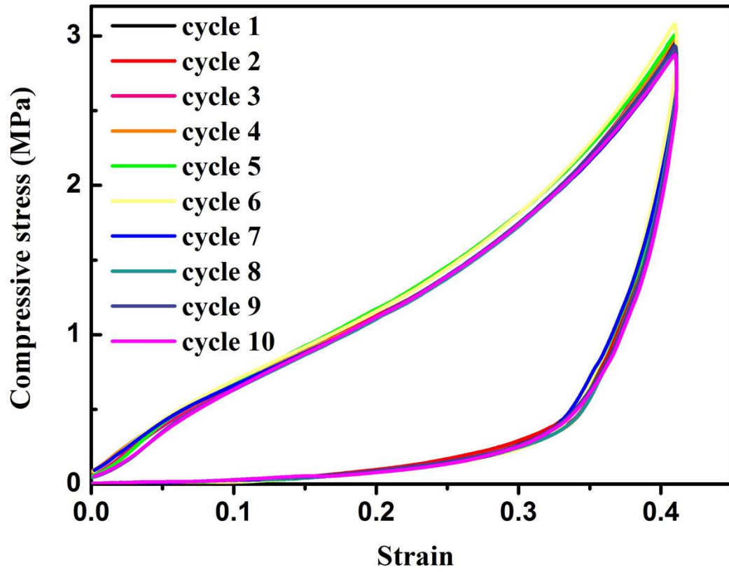
Figure S1 | 10 cycles of measured loading and unloading curves for the rubber
