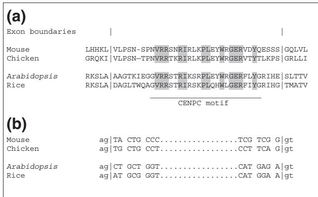
Figure S1 Conservation of the exon containing the CENPC motif. (a) Alignment of amino-acid sequences encoded by exons containing the CENPC motif in mouse, chicken, Arabidopsis , and rice. (b) The flanking splice junctions are positioned in the +1 reading frame.
