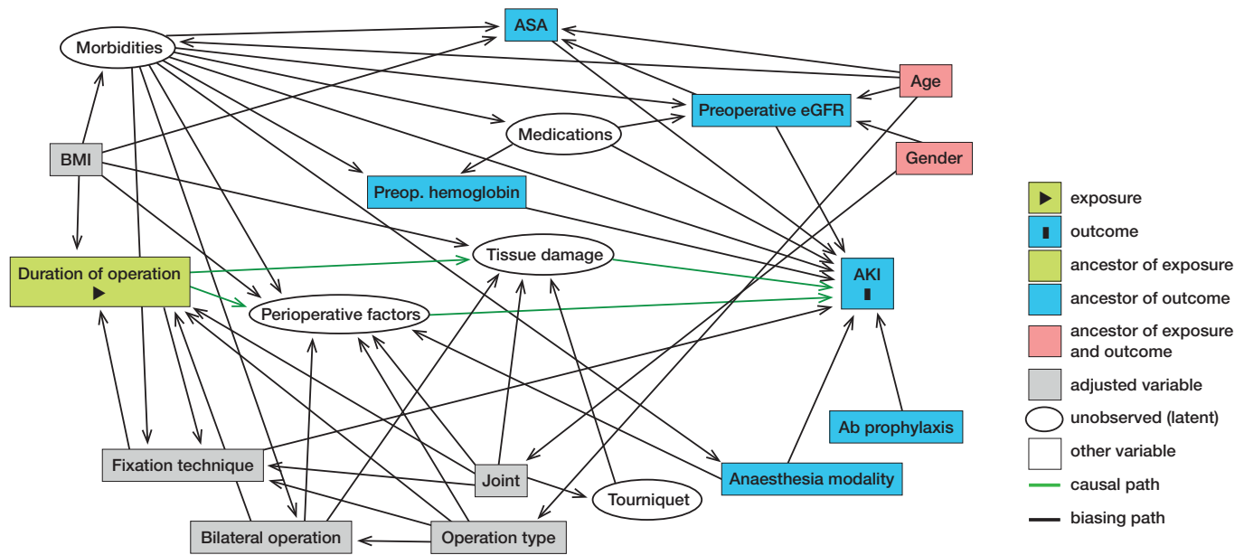
Directed acyclic graph.
