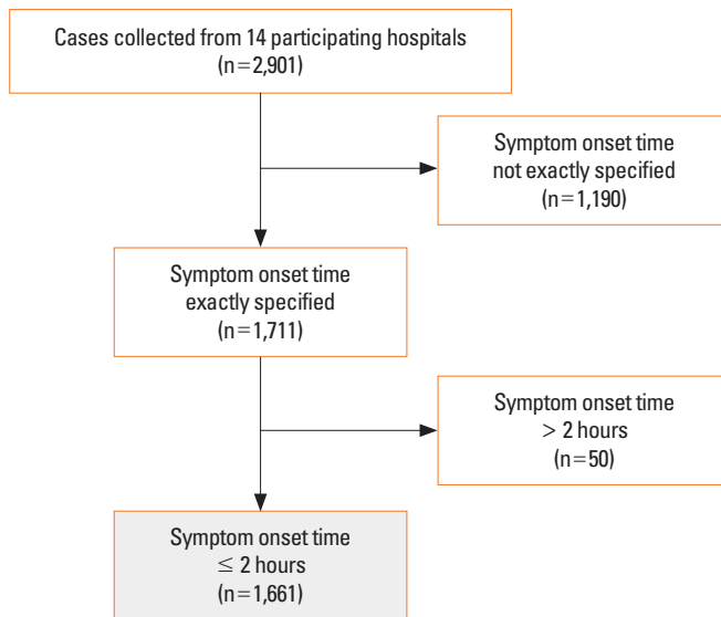
Supplementary Fig. 1. Flow-chart for case selection according to symptom onset time.
