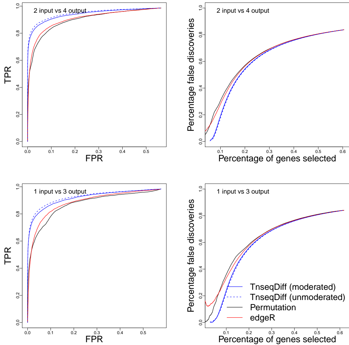
Figure1S: Evaluate the model performance for identifying conditionally essential genes. ROC curves (left) where y axis is the true positive rate and x axis is the false positive rate and False discovery curves (right) where y axis is the percentage false discoveries and x axis is the percentage of selected genes. Four methods applied to 20 simulated datasets and results are summarized over all datasets.
