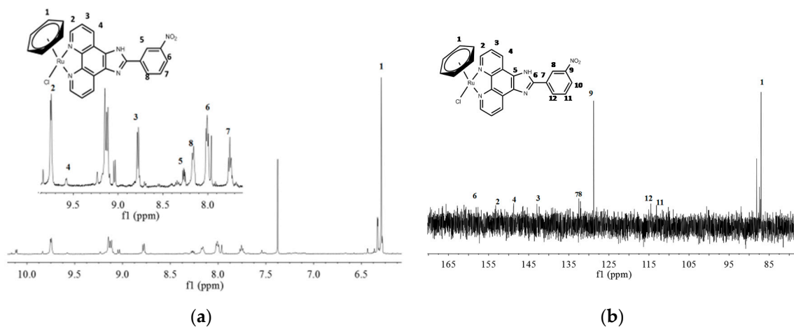
Figure S5. The ^1\text{H} NMR (a) and ^{13}\text{C} NMR (b) spectra of complex 4b .
