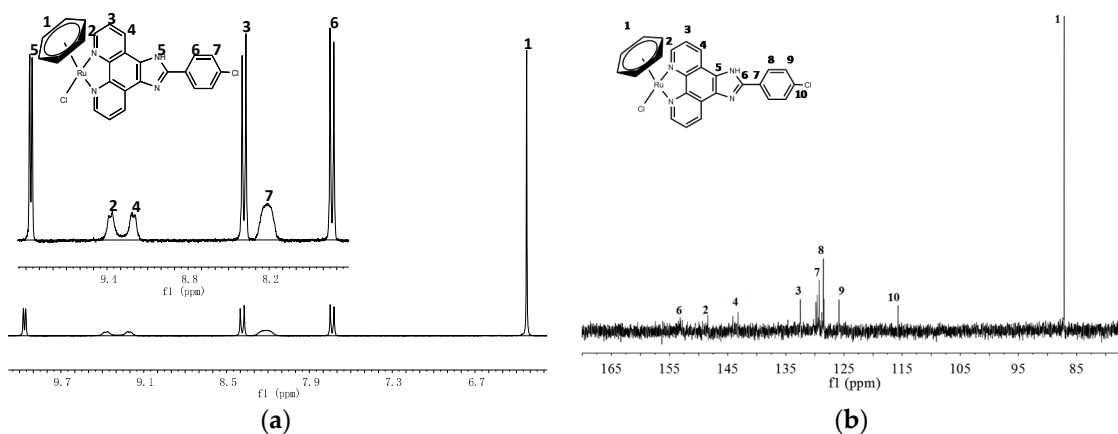
Figure S2. The ^1\text{H} NMR (a) and ^{13}\text{C} NMR (b) spectra of complex 1b.
