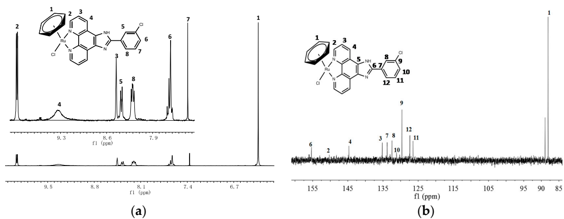
Figure S3. The ^1\text{H} NMR (a) and ^{13}\text{C} NMR (b) spectra of complex 2b .
