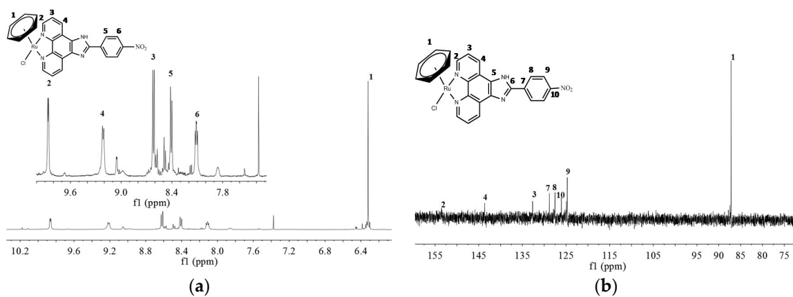
Figure S4. The ^1\text{H} NMR (a) and ^{13}\text{C} NMR (b) spectra of complex 3b .
