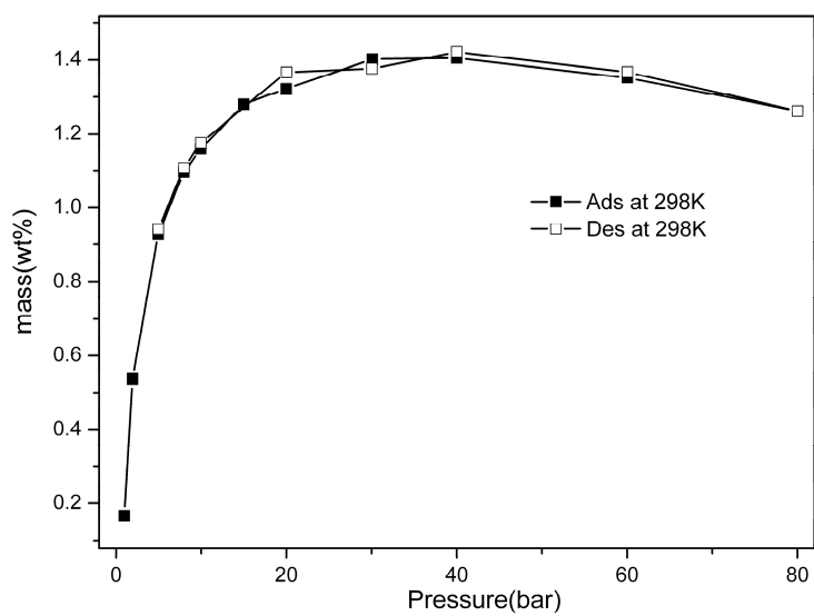
Figure S3. Methane adsorption isotherm of Zn(hfipbb) at 298 K.
