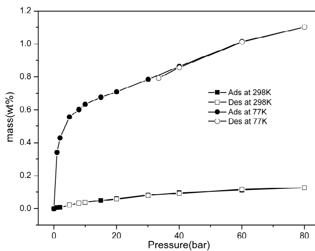
Figure S2. Hydrogen adsorption isotherms of Zn(hfipbb) at 77 K and 298 K.
