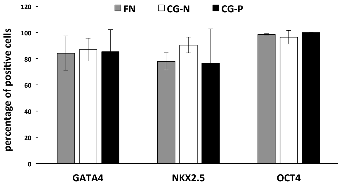
Supplementary figure 1: Quantification of immunofluorescence staining. Bargraph shows the percentage of cells positive for GATA4, NKX2-5 and OCT4 as per immunostaining shown in figure 3.
