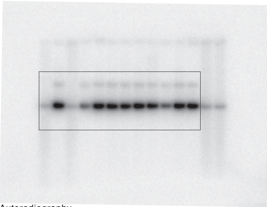
Autoradiography
