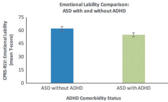
SUPPLEMENTARY FIG. S3. Group mean EL scores (CPRS-RLV; T -score) do not differ between children with ASD with comorbid ADHD and those without comorbid ADHD. ADHD, attention-deficit/hyperactivity disorder; ASD, autism spectrum disorder; CPRS-RLV, Conners Parent Rating Scale- Revised-Long Version.
