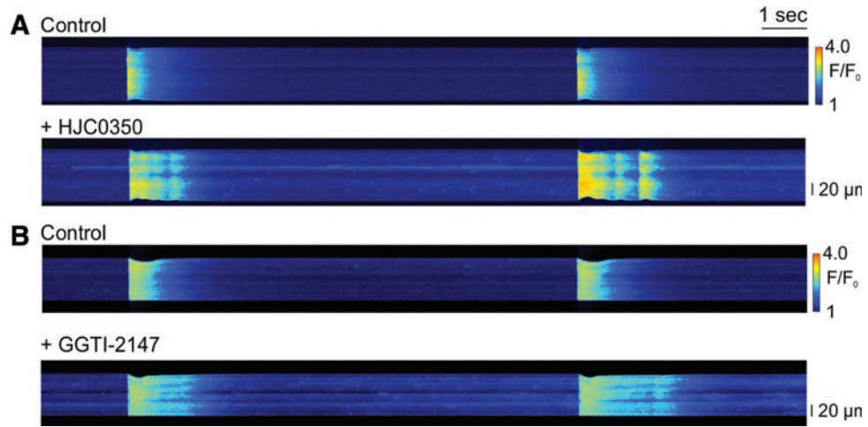
SUPPLEMENTARY FIG. S1. Effects of HJC0350 and GGTI-2147 on the electrically stimulated [Ca^{2+}]_i . (A) Typical effect of the Epac2 inhibitor, HJC0350 ( 10 \mu M ), on the electrically stimulated [Ca^{2+}]_i transient measured in fluo-4-loaded ARVMs. Similar results were obtained in four other cells. (B) Typical effect of the GGT-1 inhibitor, GGTI-2147 ( 5 \mu M ), on the [Ca^{2+}]_i transient. Similar results were obtained in four other cells.
