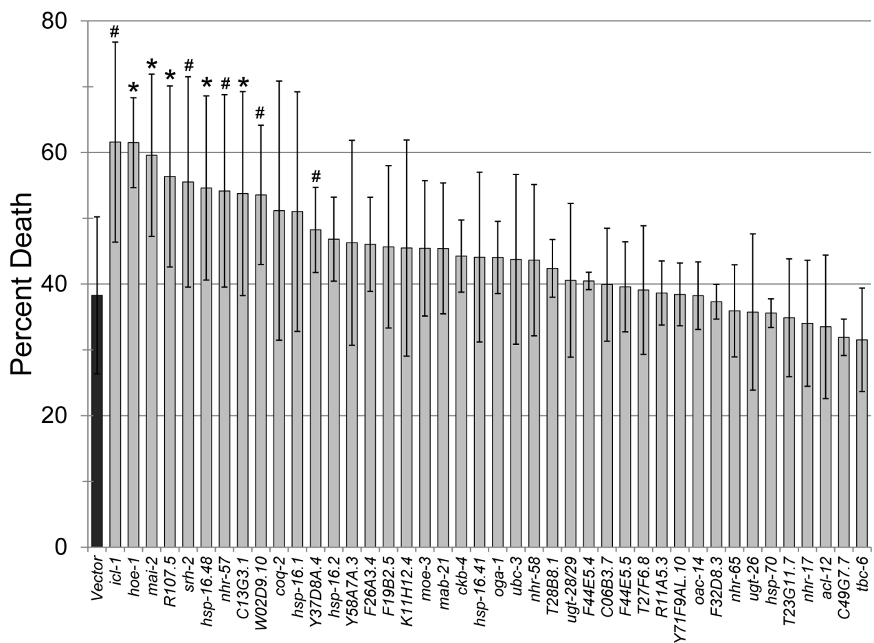
S4 Fig. A subset of ESRE genes is necessary for survival during Liquid Killing
