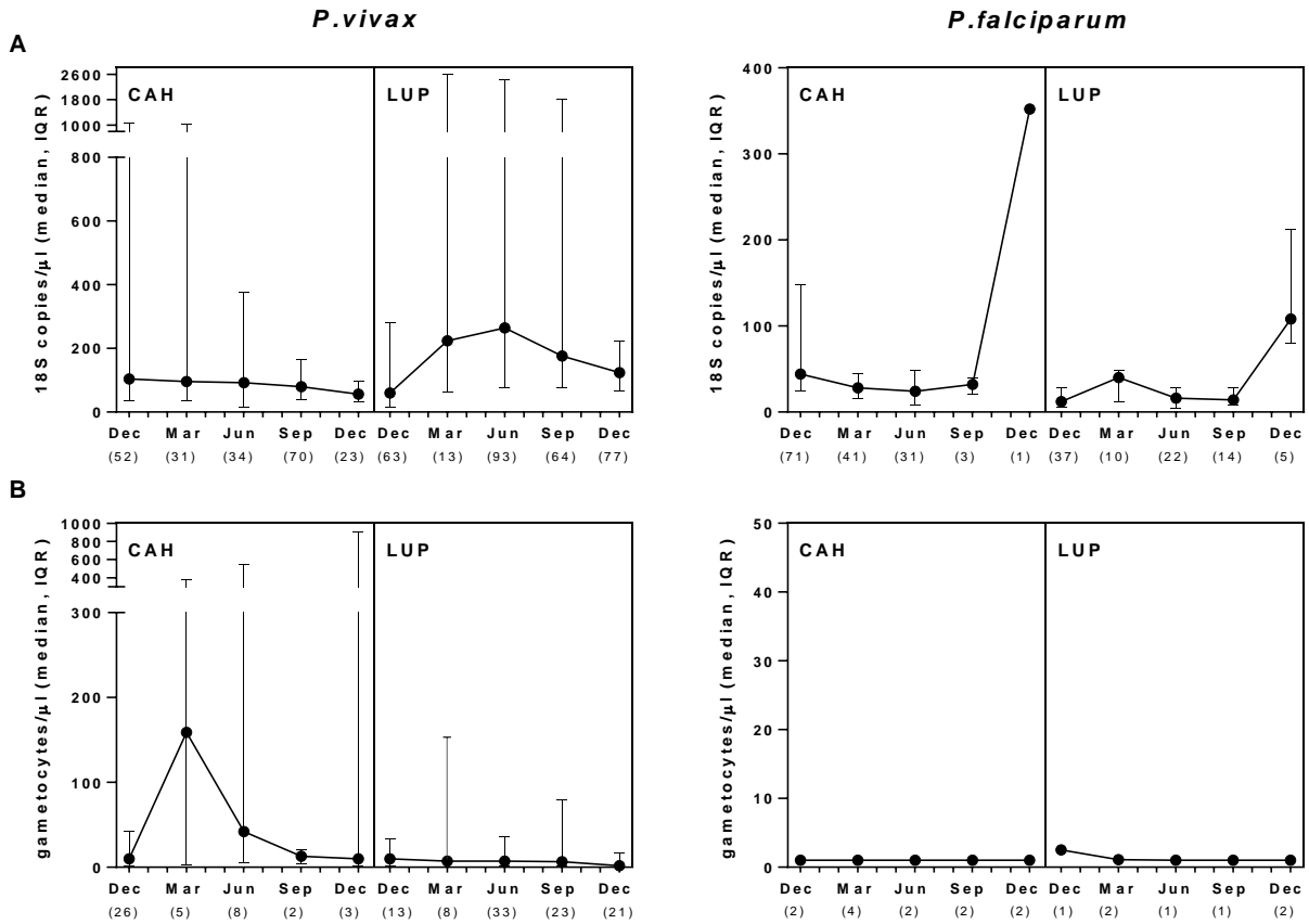
S1 Fig. Plasmodium densities by qPCR/RTqPCR. A) P.vivax and P.falciparum parasite densities by qPCR as 18S rRNA copy numbers/ \mu l of blood. B) P.vivax and P.falciparum gametocyte density estimates as gametocytes/ \mu l of blood by RTqPCR. Numbers in brackets indicate number of observations at each survey.
