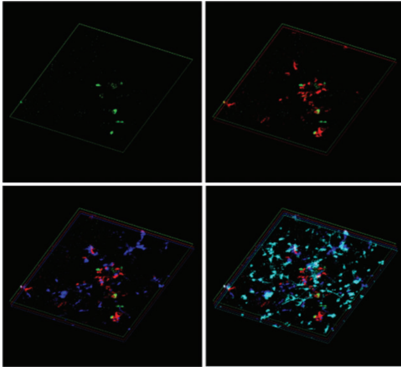
SUPPLEMENTARY FIG. S1. Representative three-dimensional (3D) OPC image. Each layer (different color of OPCs) is displayed at intervals of 30 \mu\text{m} from top to bottom from consecutive cross-section images (PDGF-R \alpha staining on day 3) of our OPCs. OPC, oligodendrocyte precursor cell; PDGF-R \alpha , platelet-derived growth factor receptor \alpha .
