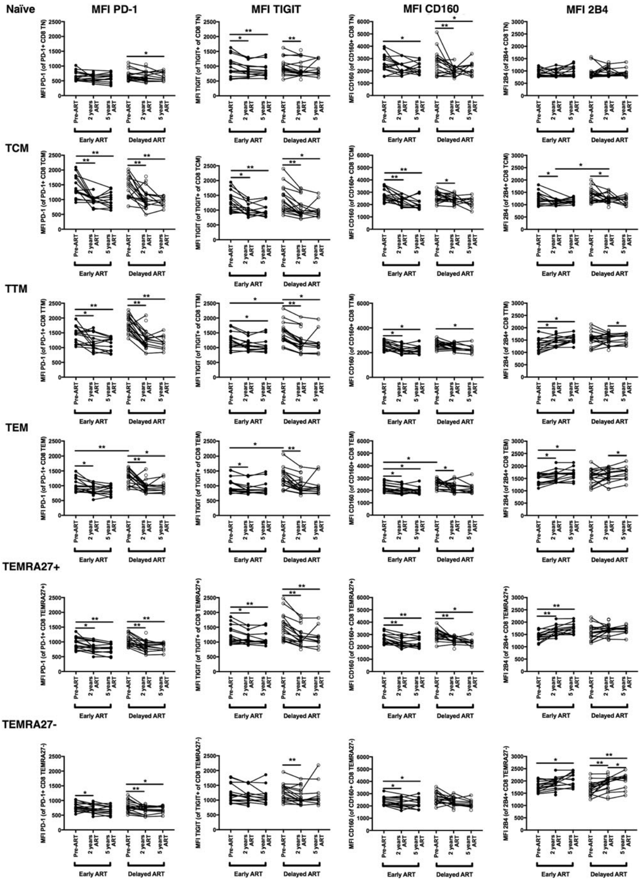
SUPPLEMENTARY FIG. S2. Exhaustion marker expression (MFI) in all CD8 + T cell subsets. The MFI of the cells that fall within the positive gate for the four exhaustion markers is shown. * p < .05, ** p < .01. MFI, median fluorescence intensity.
