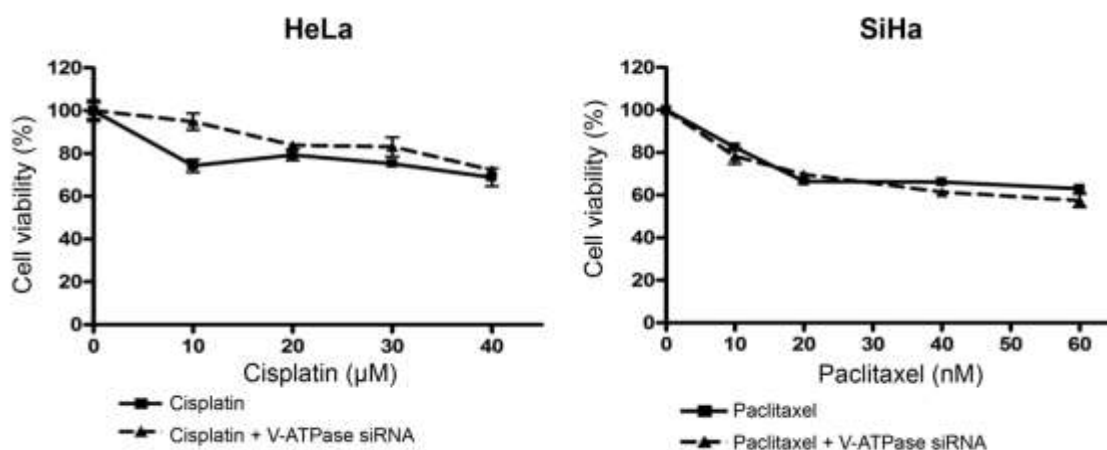
S3 Fig. (A) Effects of vacuolar-type \text{H}^+ ATPase (V-ATPase) siRNA transfection on cell viability with cisplatin in HeLa cells. (B) Effects of V-ATPase siRNA transfection on cell viability with paclitaxel in SiHa cells.
