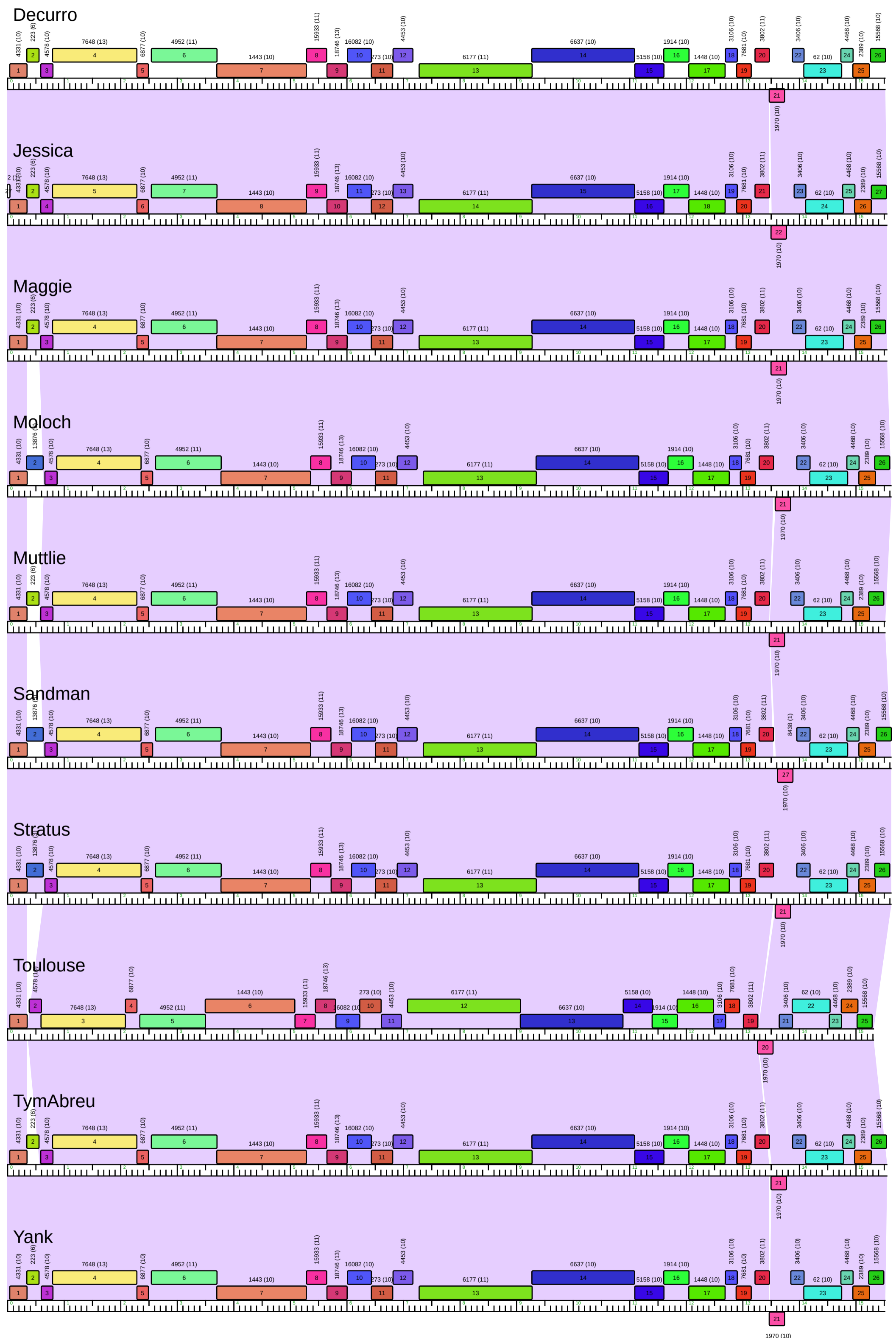
S5 Figure. Pairwise alignment of 10 Cluster AN Arthrobacter phages. See Figure 4 for details.
