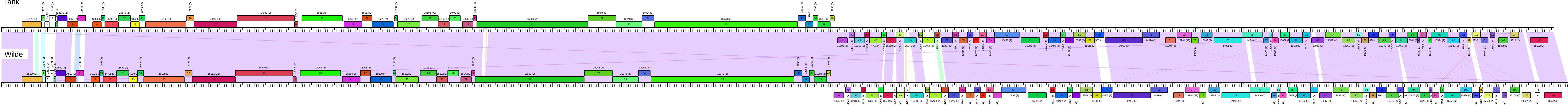
S7 Figure. Pairwise alignment of 2 Cluster AP Arthrobacter phages. See Figure 4 for details.
