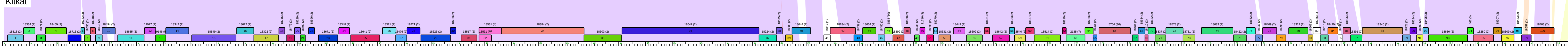
S9 Figure. Pairwise alignment of 2 Cluster AT Arthrobacter phages. See Figure 4 for details.
