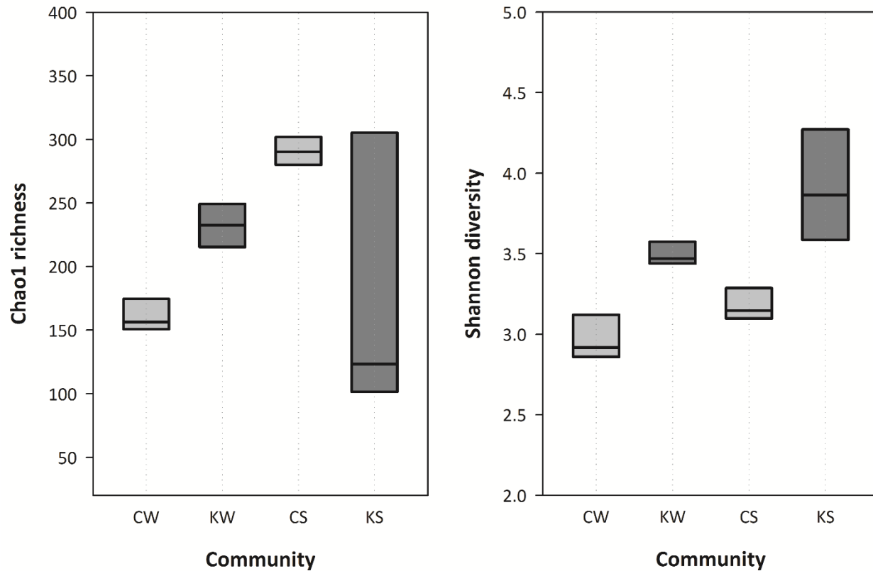
S3 Fig. Alpha diversity levels (# OTUs) of environmental microbiota in Chengcing Lake and Kaoping River after rarefaction to 20313. Chao1 richness and Shannon diversity all varied between samples from lake and river ( P < 0.001 ), except Chao1 between CS and KS ( P = 0.0388 ).
