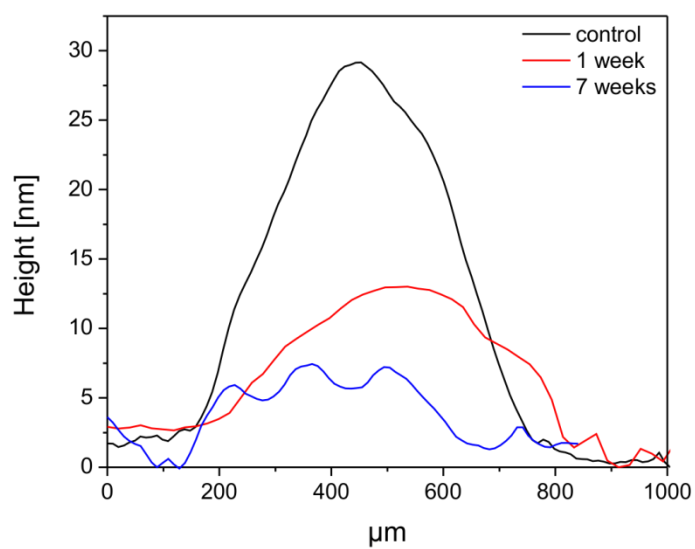
S1 Fig. Height profiles of non-degraded and partially degraded microgels pOEGMA 80/0 . After certain incubation periods the particle suspension was centrifuged onto amine-functionalized glass slides. Particles were imaged by AFM in the dried state. The control refers to the height profile of non-degraded intact particles.
