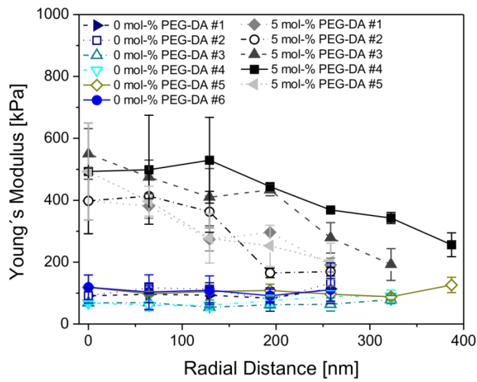
S3 Fig. Dependence of Young's modulus on the radial position within microgel. Averaged Young's modulus along the radial position starting at the particle center of PEG-DA cross-linked microgels pOEGMA 80/5 and cross-linker-free particles pOEGMA 80/0 . For each microgel type, several particles have been analyzed.
