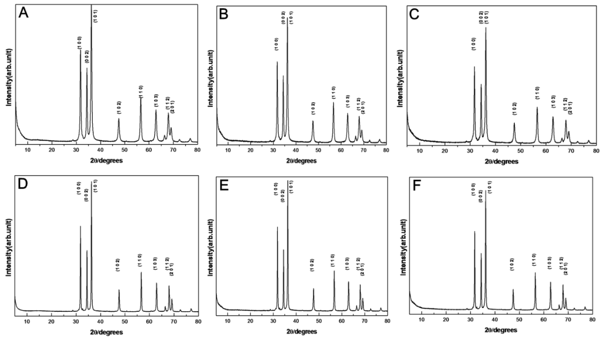
S1 Fig. X-ray diffraction patterns of the ZnO NPs. (A) Pristine 20 nm, (B) Citrate 20 nm, (C) L-serine 20 nm, (D) Pristine 100 nm, (E) Citrate 100 nm, and (F) L-serine 100 nm.
