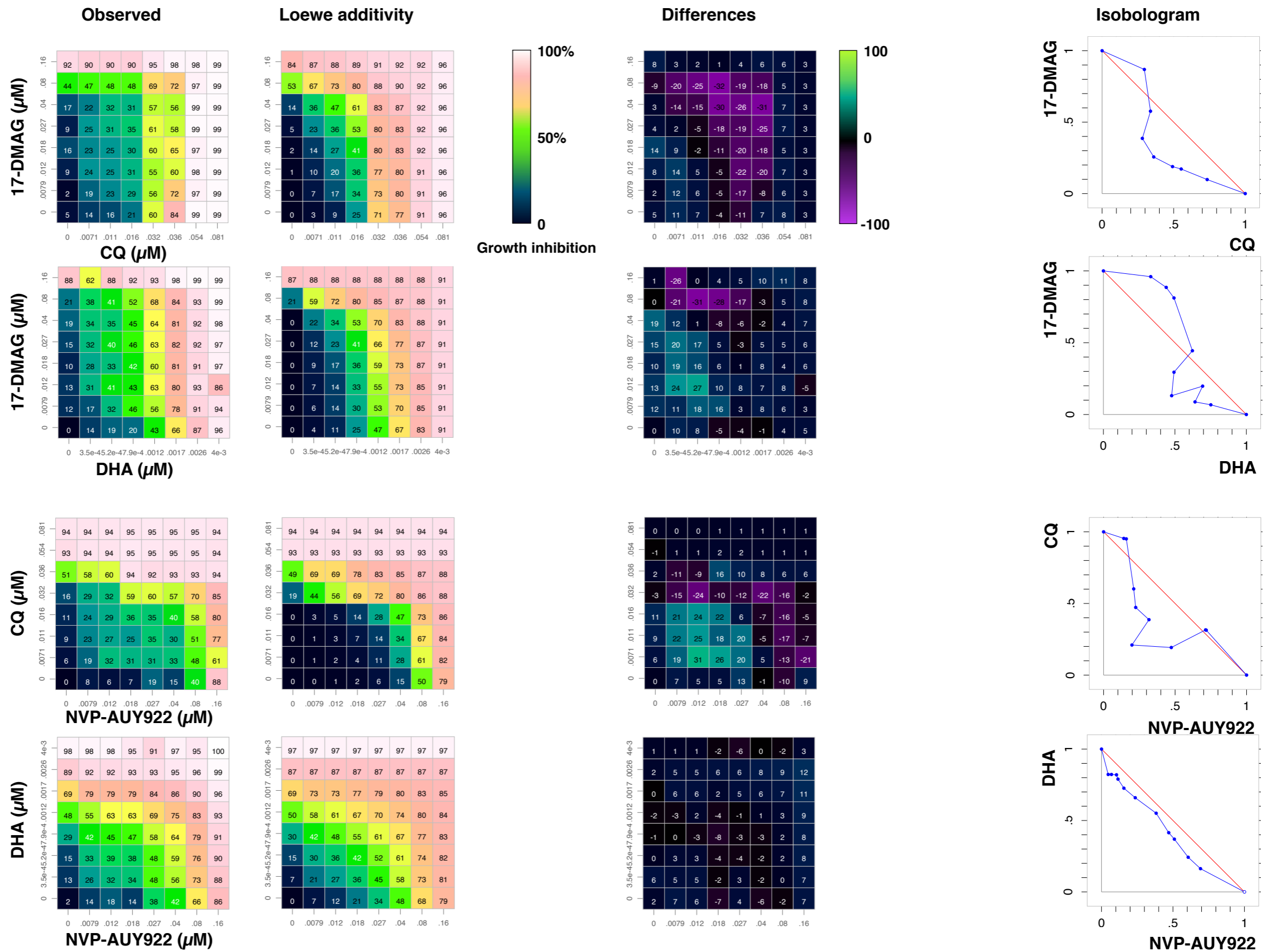
Figure S3. Hp90 and antimalarial drug combination assays for P. falciparum 3D7 strain. On the left the average of two growth inhibition experiments, the Loewe additivity expected values and the differences between the observed data and the model. On the right isobolograms obtained with the isobole line in red. The area below the red line represent synergistic interaction, above antagonistic and around it no-interaction (additive).
