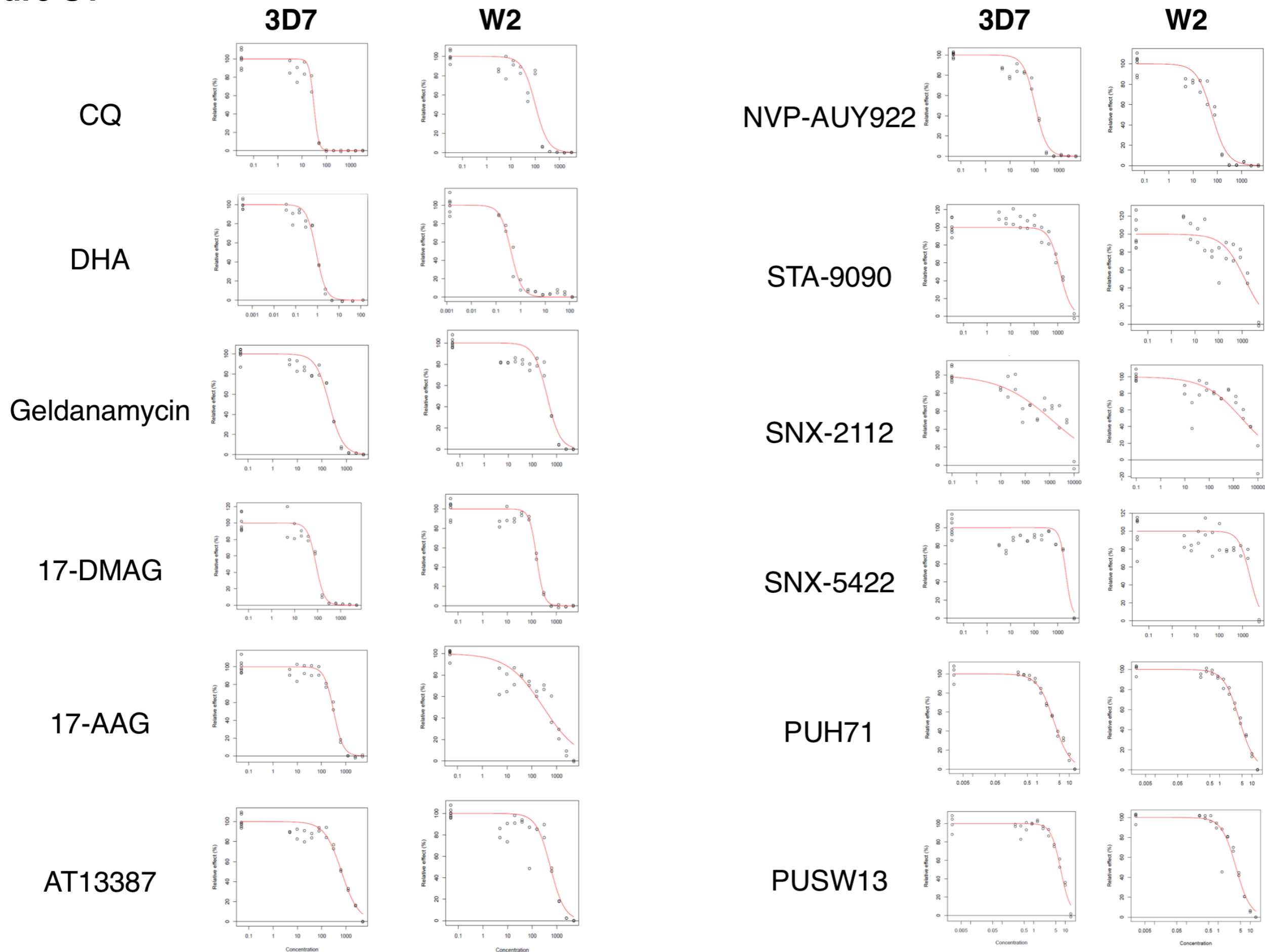
Figure S1. Dose response curves of different Hsp90 inhibitors against P. falciparum 3D7 and W2.
