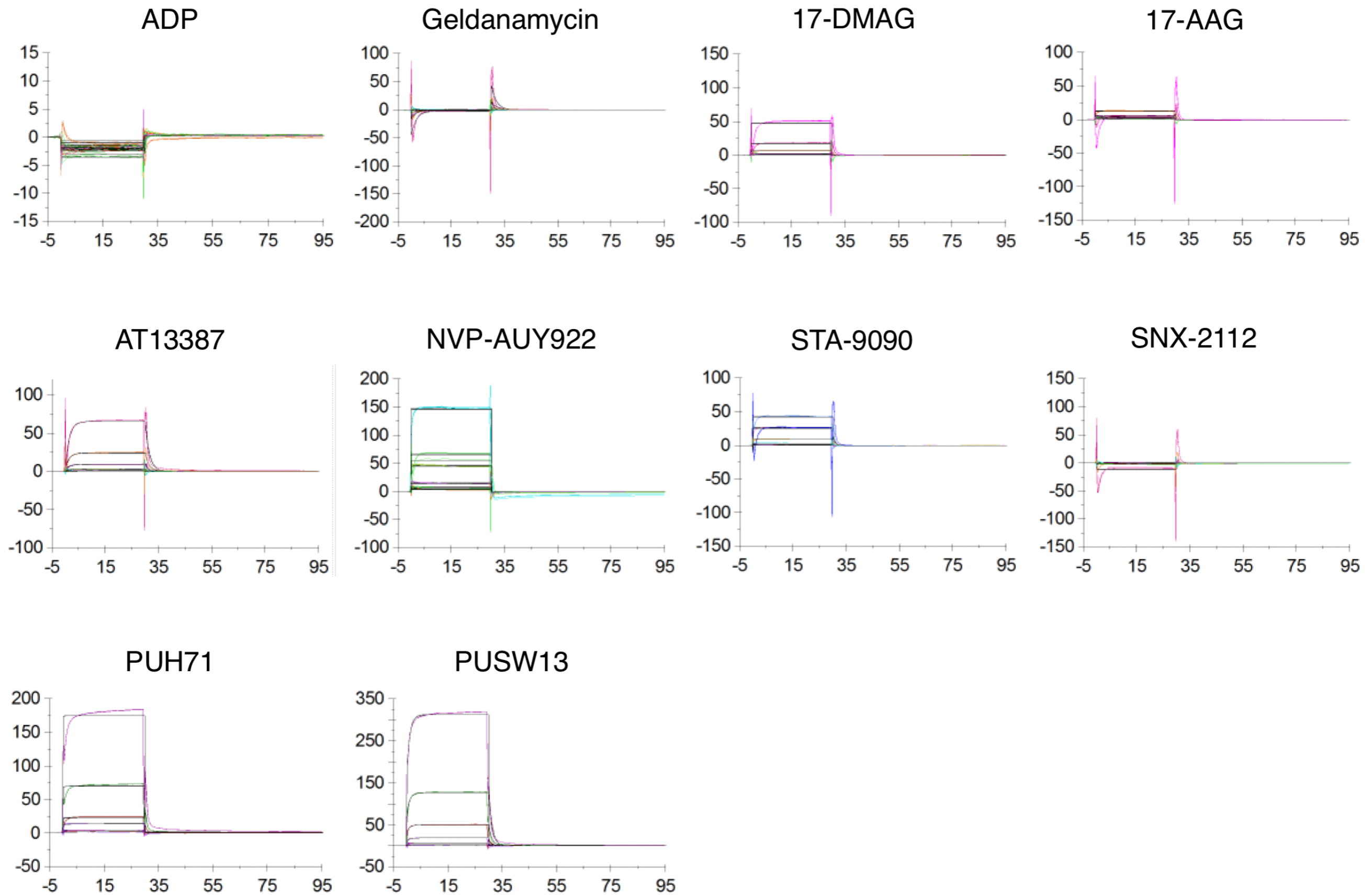
Figure S6. P. falciparum Grp94 sensorgrams of the interaction between the parasite NTD against ADP and Hsp90 inhibitors.
