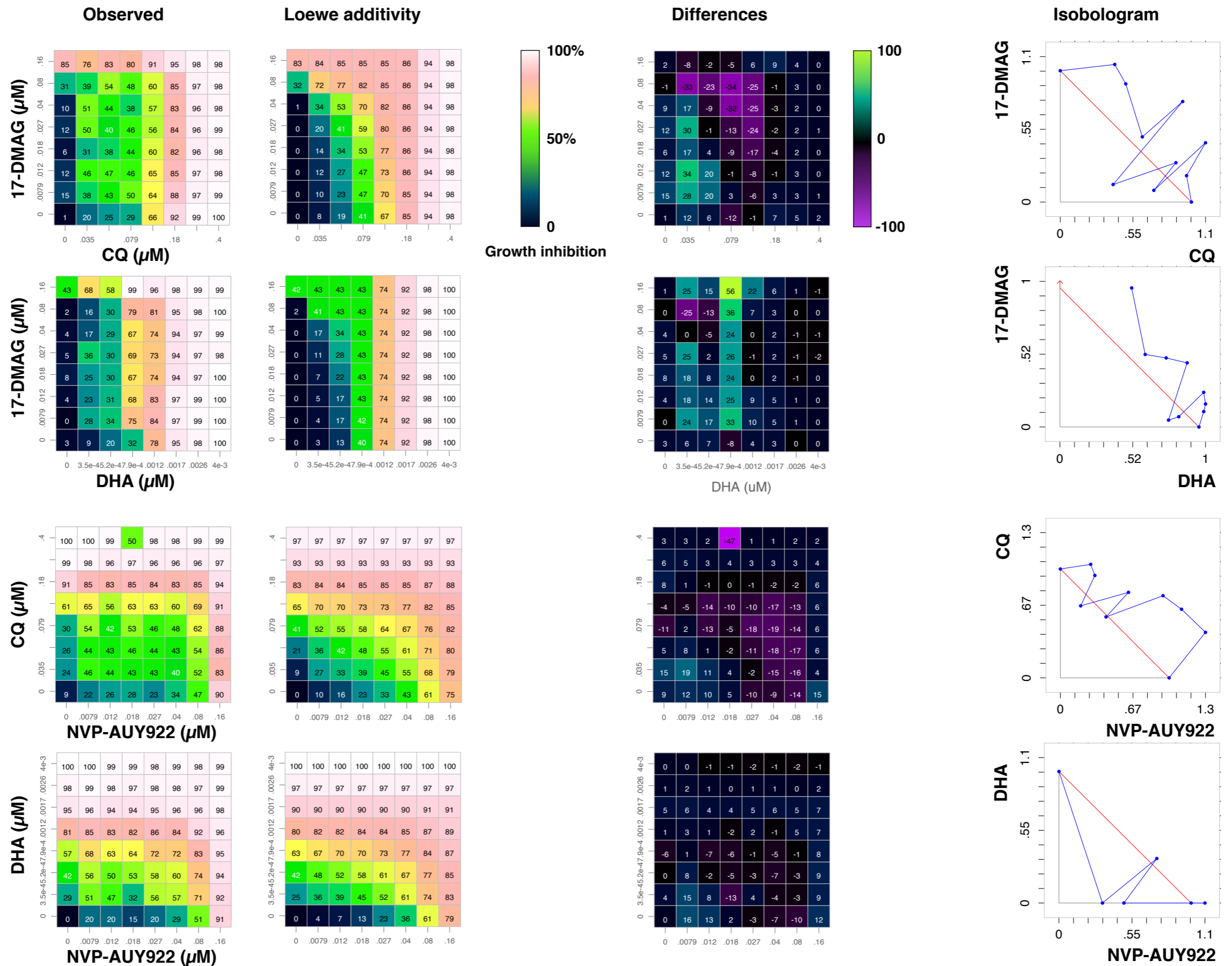
Figure S4. Hp90 and antimalarial drug combination assays for P. falciparum W2 strain. On the left the average of two growth inhibition experiments, the Loewe additivity expected values and the differences between the observed data and the model. On the right isobolograms obtained with the isobole line in red. The area below the red line represent synergistic interaction, above antagonistic and around it no-interaction (additive).
