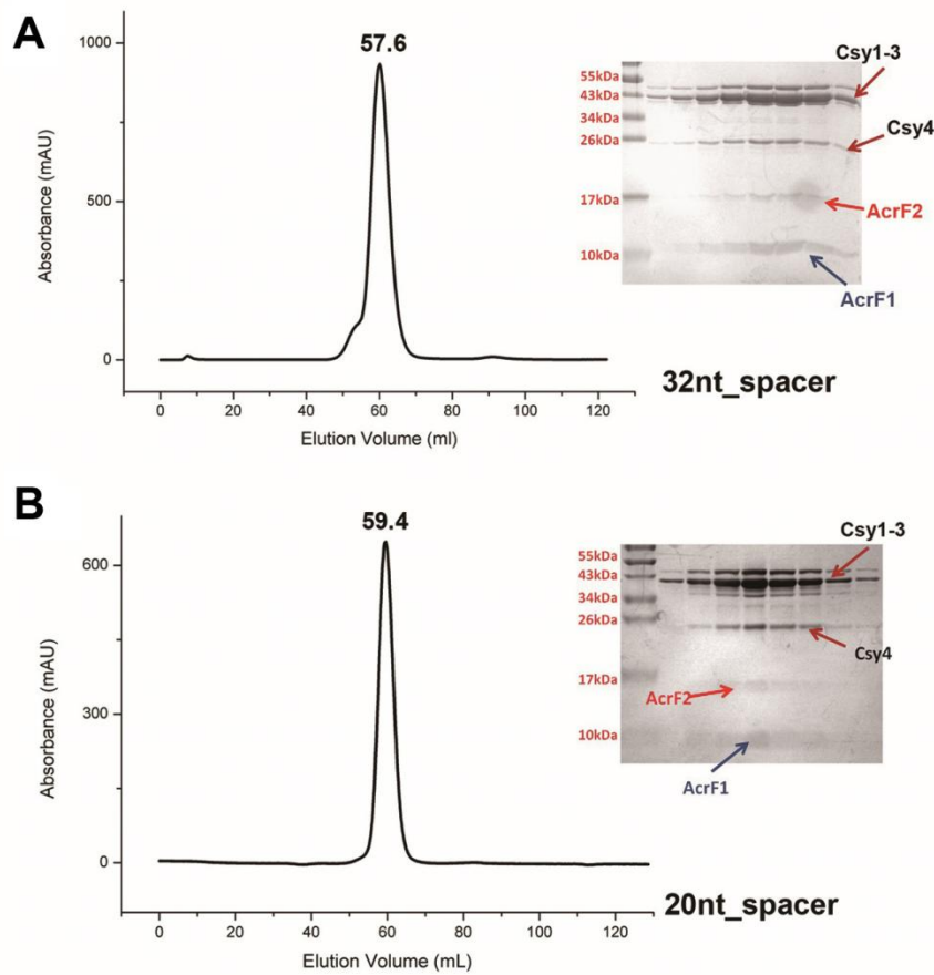
Figure S1 Size exclusion chromatogram and SDS-PAGE profiles of AcrF1/2-Csy32nt complex and AcrF1/2-Csy20nt complex . The samples were analyzed by a Superdex 200 10/600 pg size-exclusion column and eluted fractions were analyzed by SDS-PAGE. The elution volume of each sample is labeled aside the peak and all protein component bands are indicated accordingly in the SDS-PAGE photos. (A) and (B) represent the complex with 32nt and 20nt spacers, respectively.
