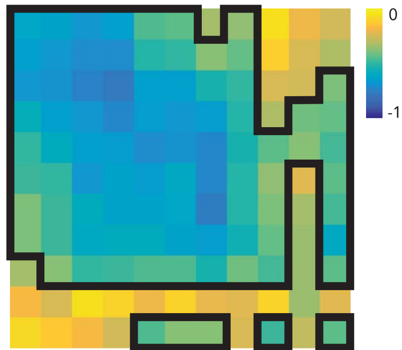
Betweenness Centrality
