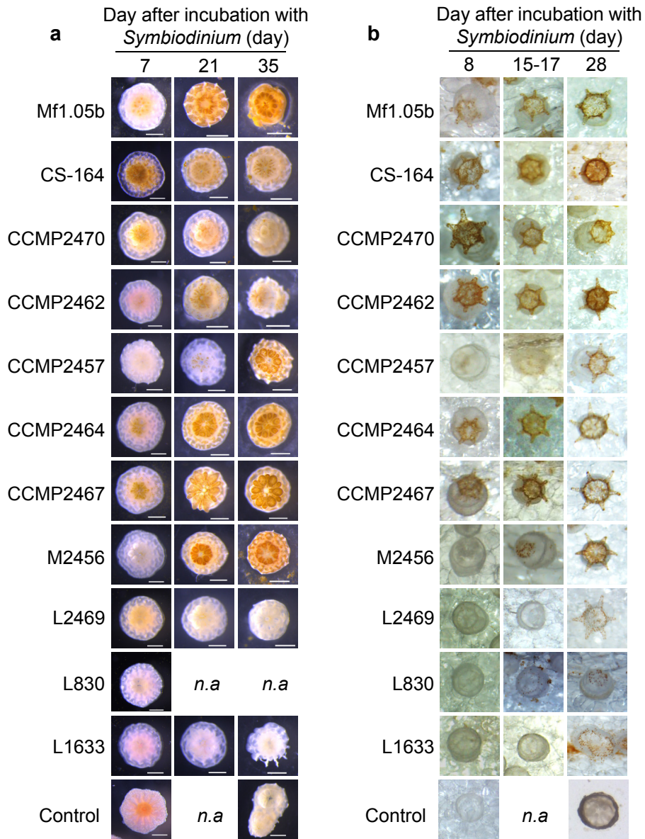
Figure S3 Infection of different Symbiodinium strains into corals. Aposymbiotic primal polyps of A. tenuis (a; scale bars, 500 \mu m) and C. serailia (b) were separately incubated with different Symbiodinium strains. Uptake of Symbiodinium into coral polyps was monitored using a stereomicroscope. Control, without Symbiodinium ; n.a., not available.
