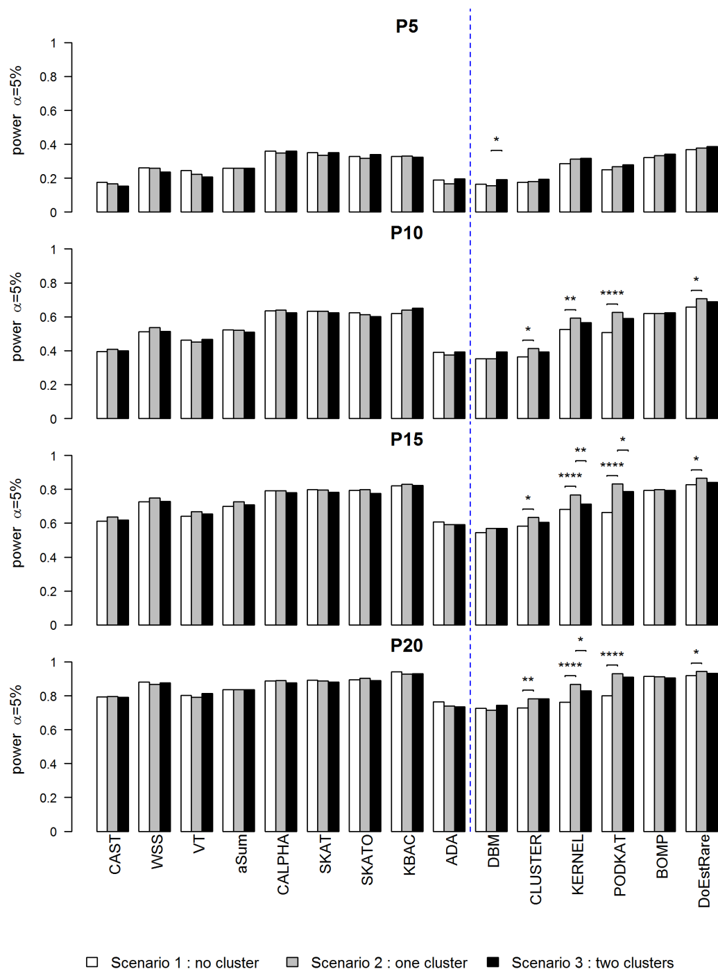
Fig A. Power comparison between scenarios. A Fisher exact test has been performed to test the independency between the gene significance at level \alpha=5\% and the compared scenarios [see S1 Text, p15]. We compared scenarios 1 and 2 (resp. 2 and 3). ns: p>0.05 , *: p\leq 0.05 , **: p\leq 0.01 , ***: p\leq 0.001 , ****: p\leq 0.0001 . The dashed blue line separates “position tests” (DBM, CLUSTER, KERNEL, PODKAT, BOMP and DoEstRare) from other tests.
