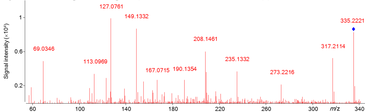
Figure S10. MS/MS spectrum for peak a) from COX-2 enzymatic hydroxylation of the (±)-8,9-EET
