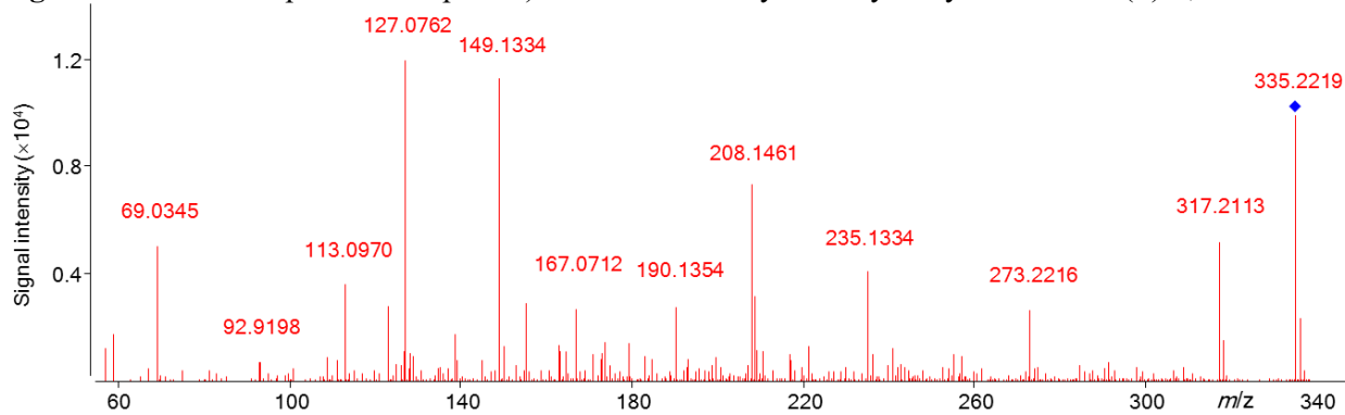
Figure S11. MS/MS spectrum for peak b) from COX-2 enzymatic hydroxylation of the (±)-8,9-EET
