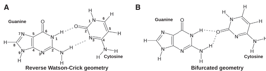
FIGURE 1 Schematic representation of the (A) RWC and (B) bifurcated geometries of the Levitt basepair. Hydrogen bonds are shown as dashed lines.
