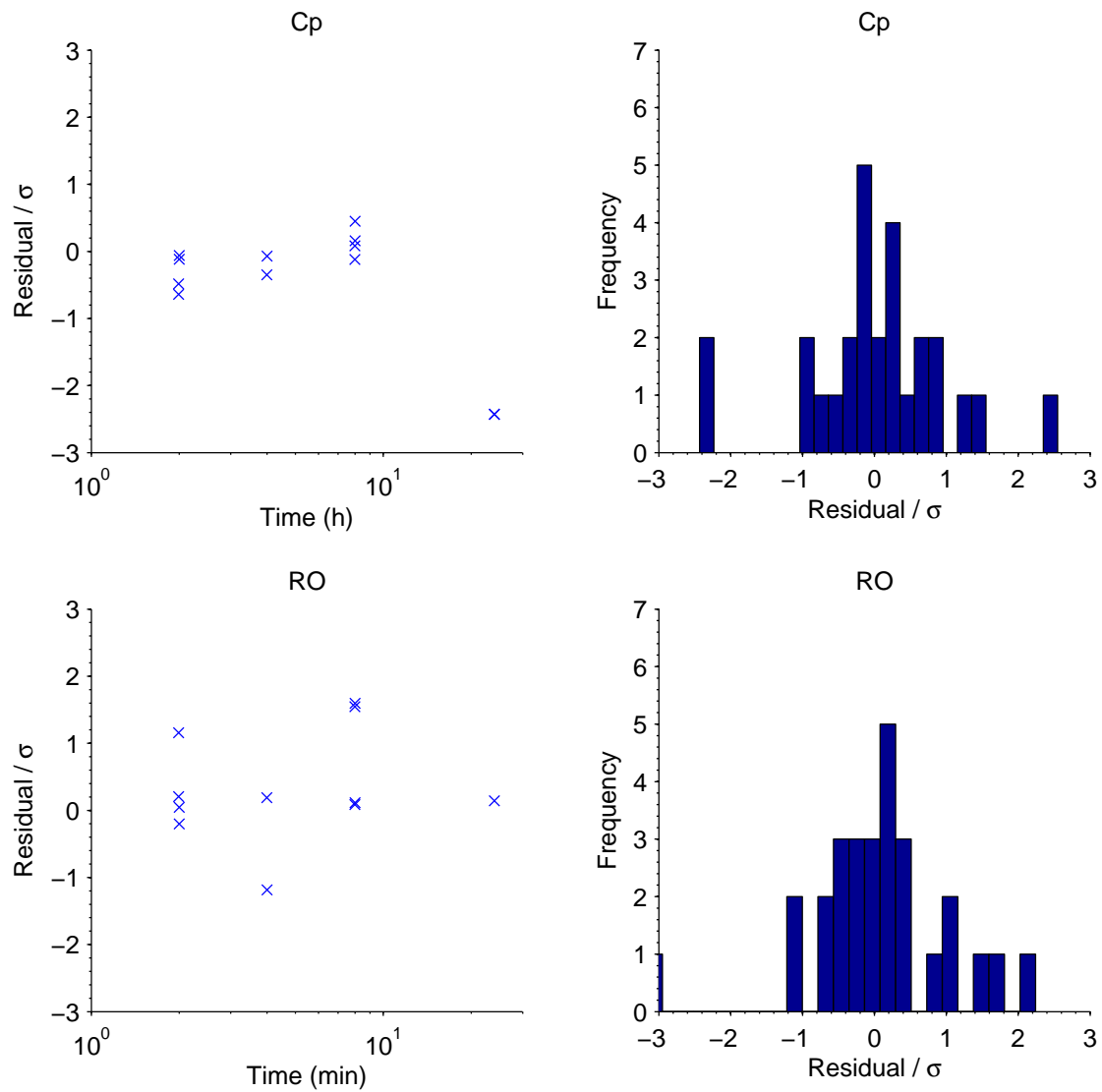
Supplementary Figure 5. Residual plots corresponding to the model fit in Figure 4. Each row corresponds to one observed variable. The left column displays residuals divided by the estimated \sigma for each variable, and over sampling times. The right column shows the corresponding histograms for the residuals, collected over all sampling points.
