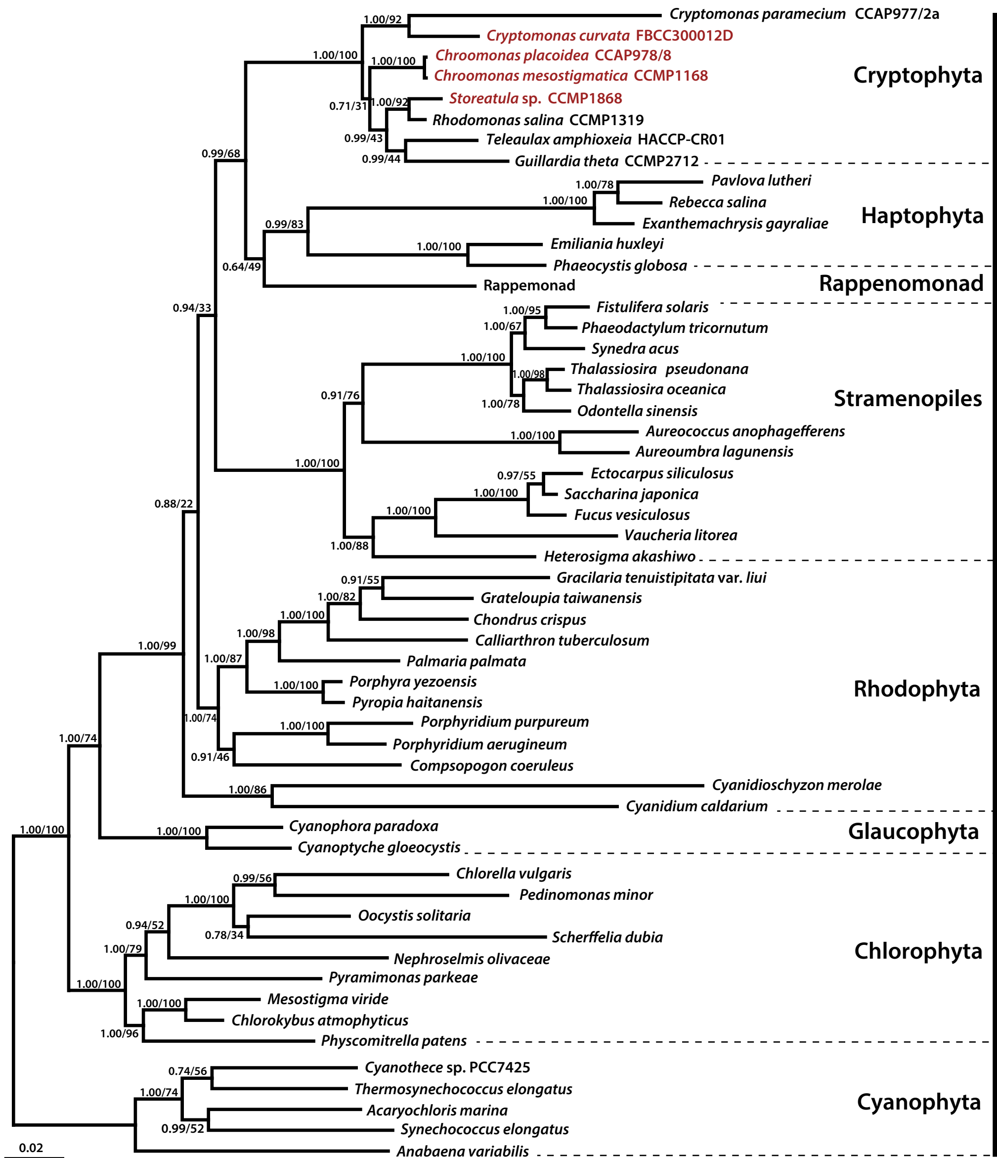
Figure S13. Bayesian tree based on RNA operon (16S-trnI-trnA-23S) sequences.
