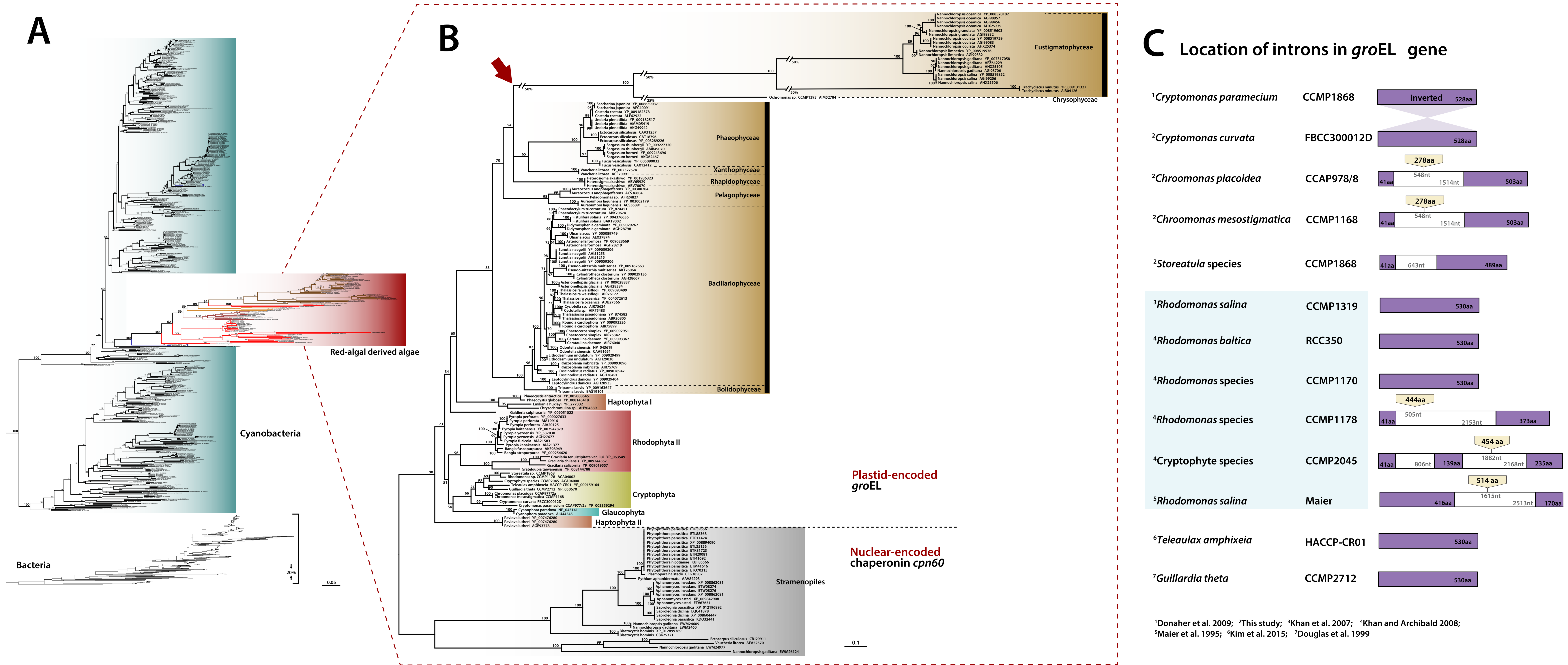
Figure S3. Phylogenetic tree based on groEL .
