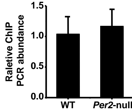
Supplement Figure 2 Effect of Per2 deficiency on recruitment of SP1 to Atp1a1 promoter. (A) Quantitative PCR amplification of Atp1a1 promoter detected by a ChIP assay in WT and Per2 -null bone marrow cells. All data \bar{X} \pm \text{SD} ; n=4 in each group, * p < 0.05 .
