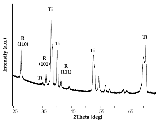
Figure S3. GAXRD spectrum of TNN475
