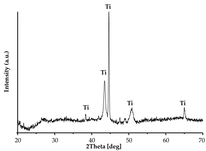
Figure S1. GAXRD spectrum of TNT20
