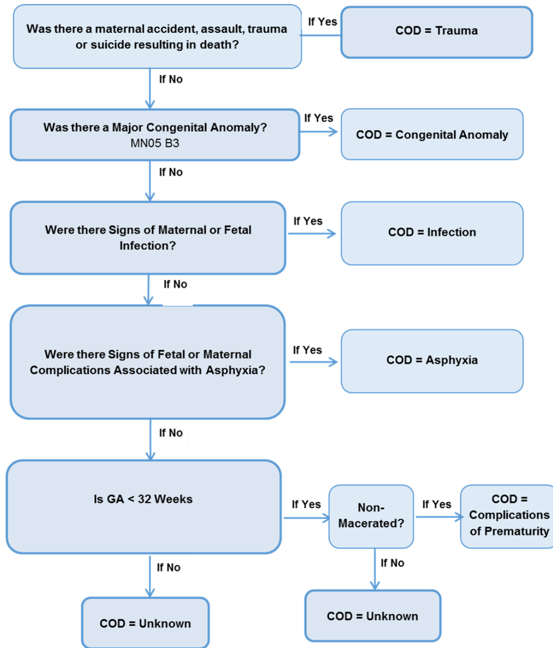
Figure S1. Global Network cause of stillbirth algorithm
