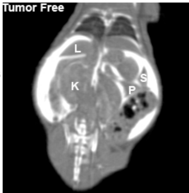
Supplementary Figure 1 CT scans of normal and tumor bearing mice, obtained using IP injection of Iohexol (4 ml)
