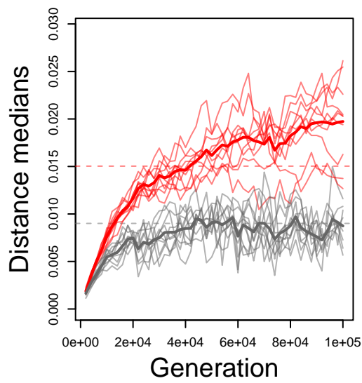
Habitat overlap 40%
