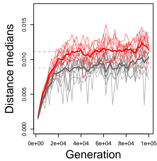
Habitat overlap 60%
