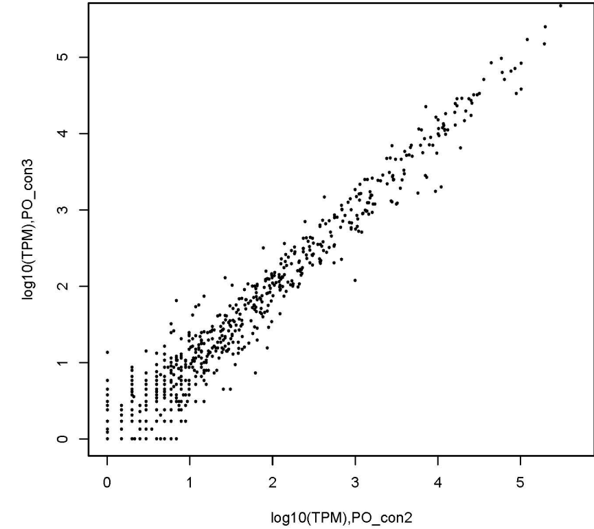
PO_con2vsPO_con3,R=0.948163394702557
