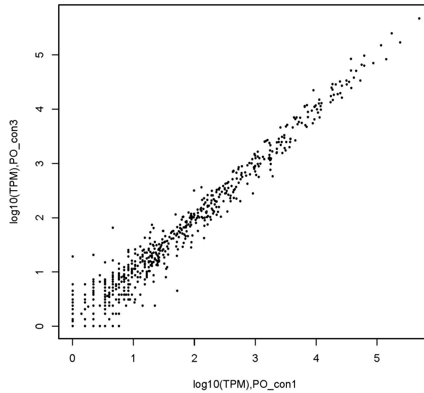
PO_con1vsPO_con3,R=0.97107208271658
