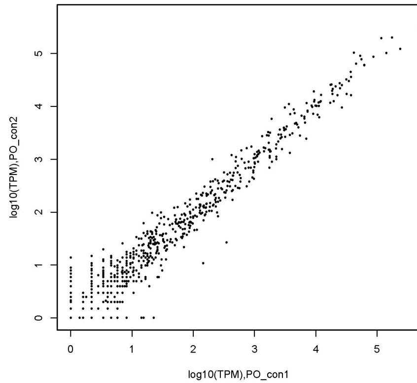
PO_con1vsPO_con2,R=0.913756934209462
