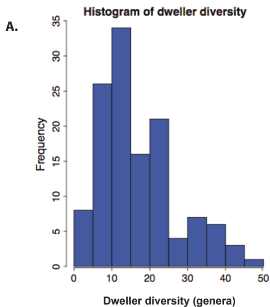
S1 Fig. Results of descriptive statistics for analysis of CCA contribution to reef dweller diversity
