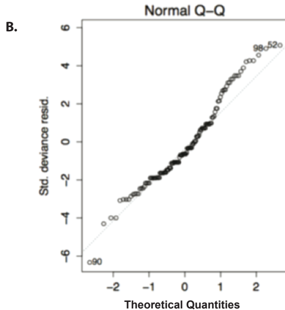
S1 Fig. Results of descriptive statistics for analysis of CCA contribution to reef dweller diversity
