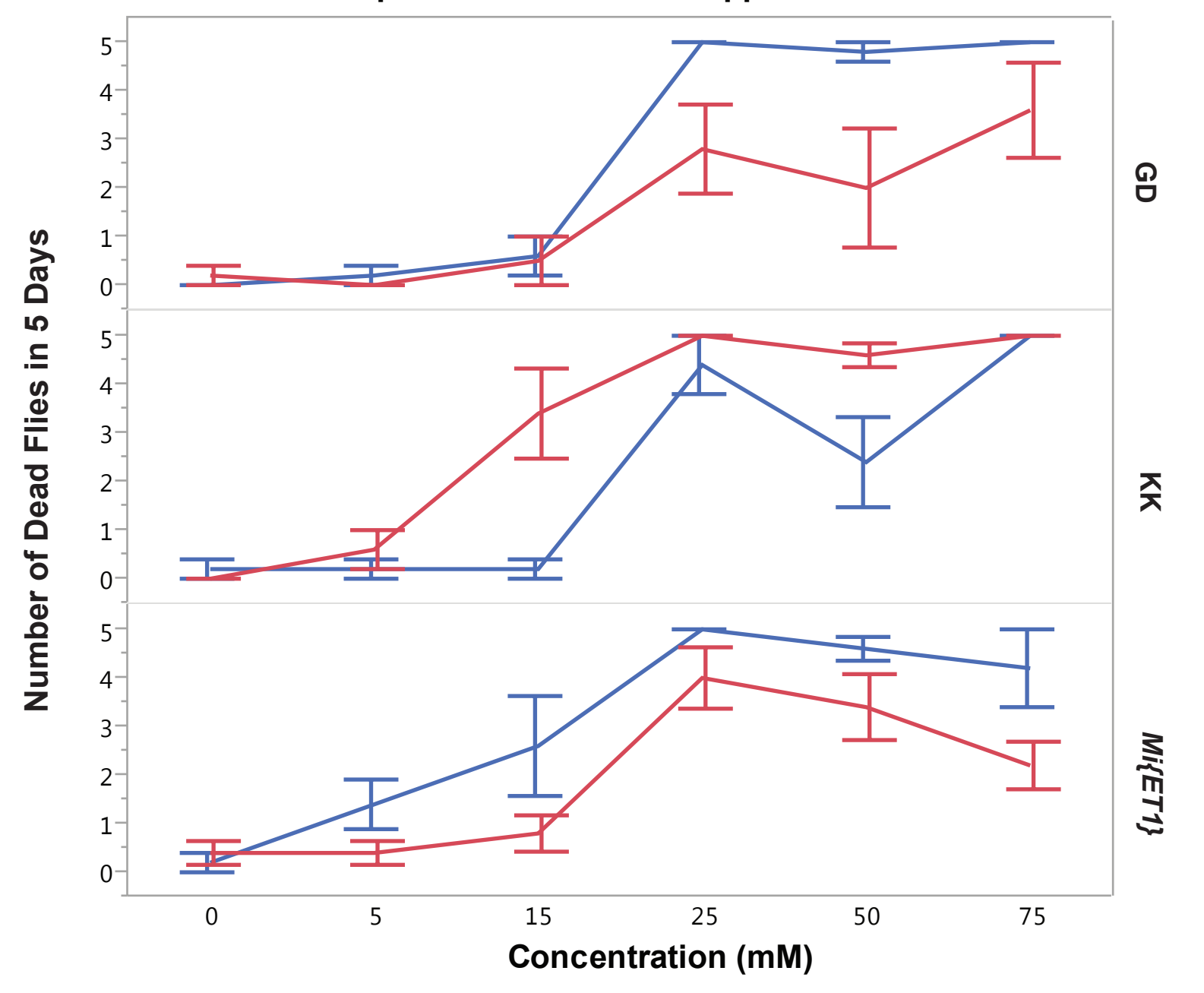
Dose-response Curve for Cd Supplemented Medium
