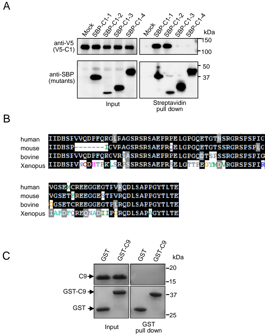
S7 Fig. Supplementary data for identification of homo-interaction regions in the MTCL1 C-terminus. (A) Streptavidin pull-down assays performed with extracts of HEK293T cells co-expressing SBP-tagged mutants and V5-tagged C1. (B) Alignment of the amino acid sequence of C9. (C) GST pull-down assays performed with a mixture of purified C9 fragment and GST or GST-C9.
